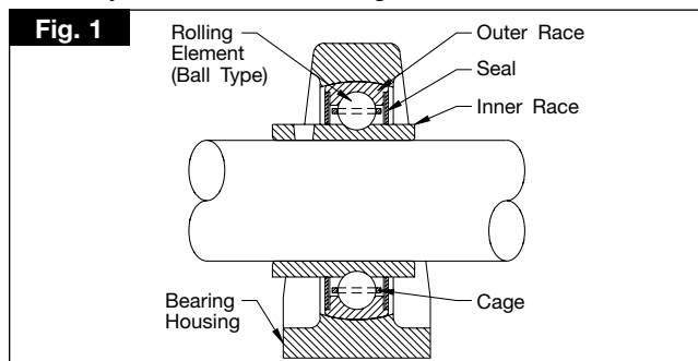
Fig. 1 Cutaway View of a Ball Bearing Unit
