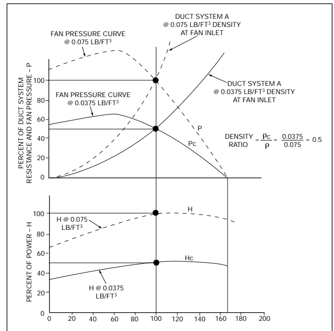
Figure 2. Percent of Duct/Fan System Airflow - Q
