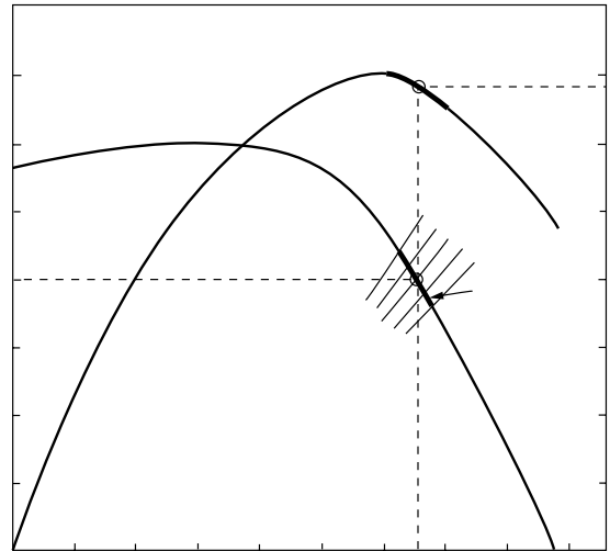
Figure 8. Variable System Characteristic Curve, Backward Inclined Centrifugal
