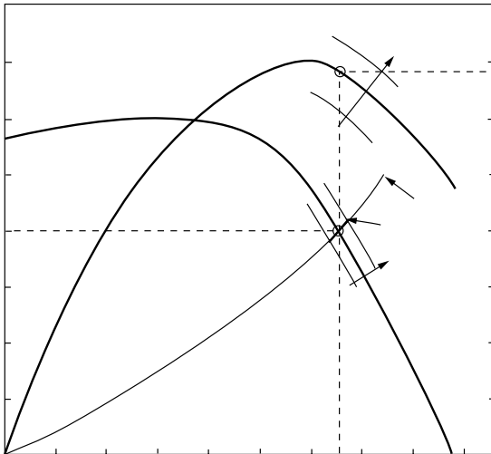
Figure 7. Variable Fan Characteristic Curve, Backward Inclined Centrifugal
