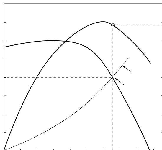
Figure 6. Fan/System Operating Point, Backward Inclined Centrifugal
