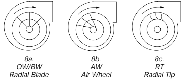
Figure 8. Common Radial Blade Impellers
