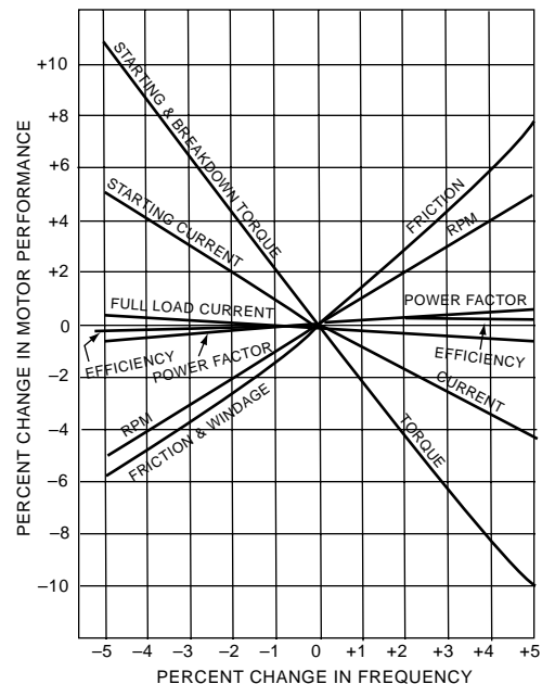
Figure 3. Frequency Variation
